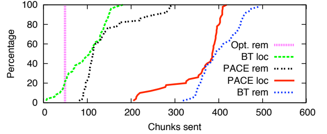
Figure 9: PACE downloaders prefer local ( loc ) to remote ( rem ) transmissions, but BitTorrent ( BT ) makes poor use of locality.
