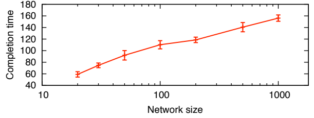
Figure 4: Completion time grows O(\log(|\text{network}|)) . Each data point shows the average performance over five runs—error bars show standard deviation—with 10 peers per cluster.
